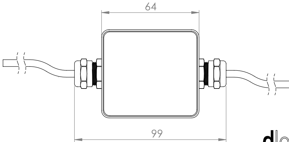
Current Splitter
